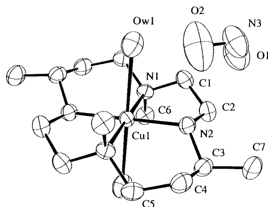
Fig. 4 An ORTEP drawing of the molecular structure of [CuL I (H 2 O) 2 ][NO 2 ] 2 3 .
