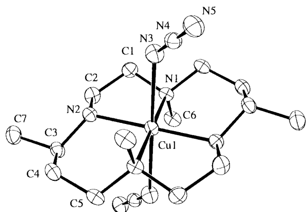
Fig. 3 An ORTEP drawing of the molecular structure of [CuL I (N 3 ) 2 ] 2 .
